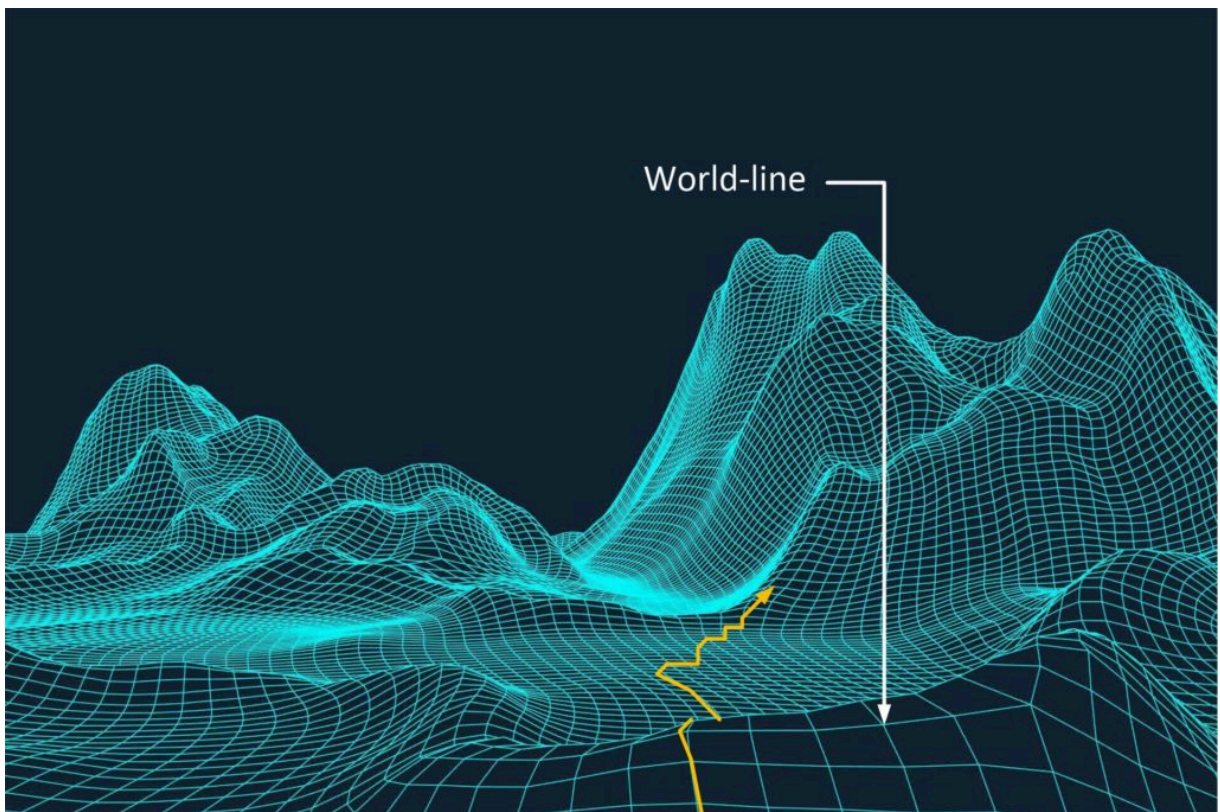
This is what a world-line is.
