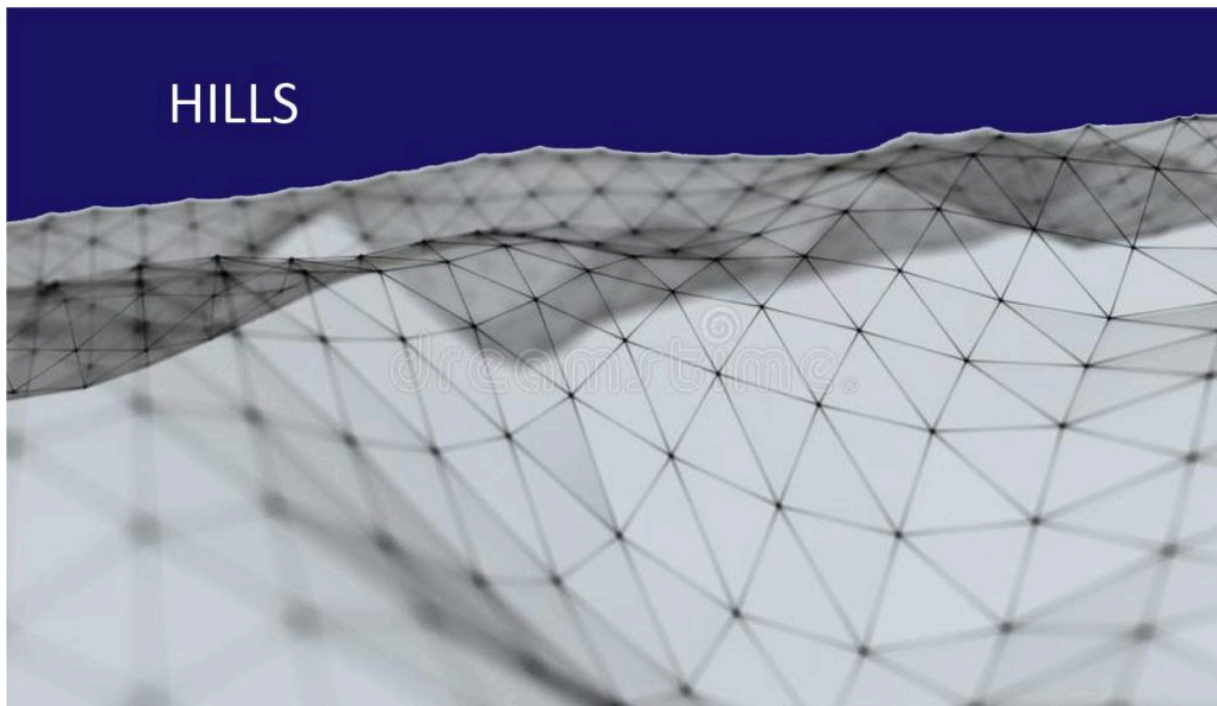
Hills on a world-line template map.
